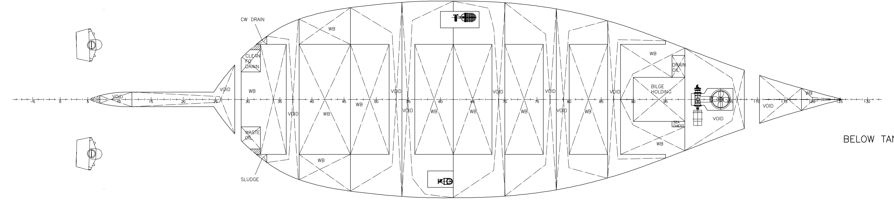
TANK TOP
