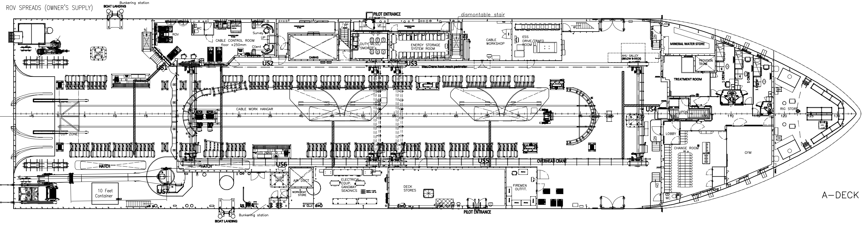
B-DECK
