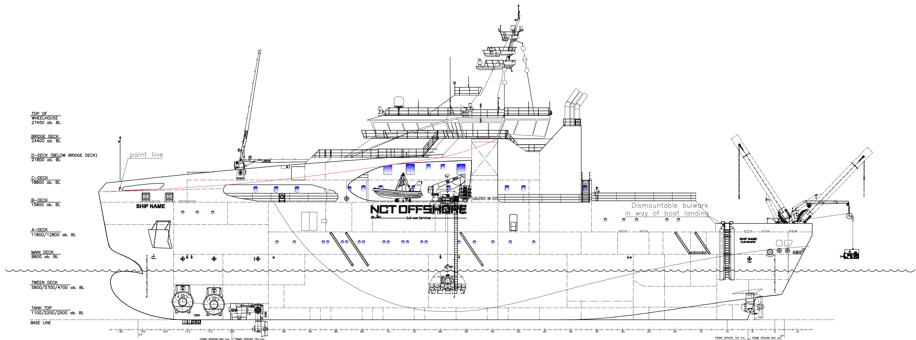
PS PROFILE
