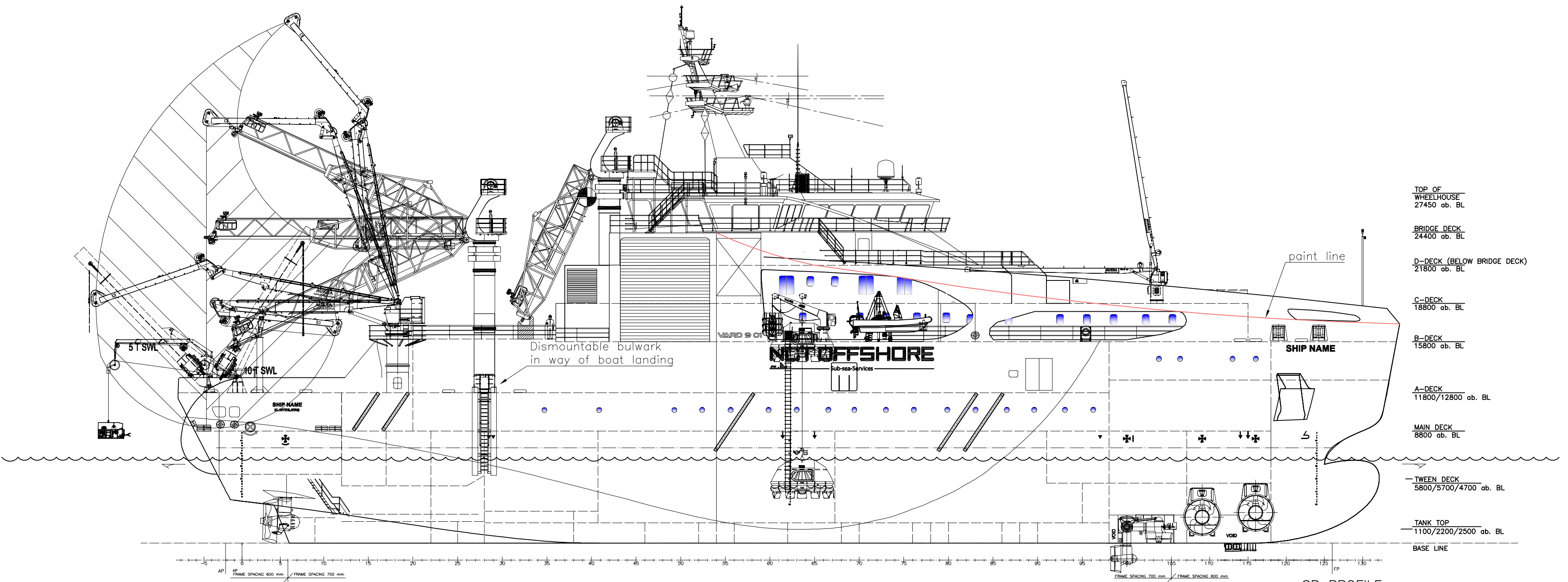
SB PROFILE
