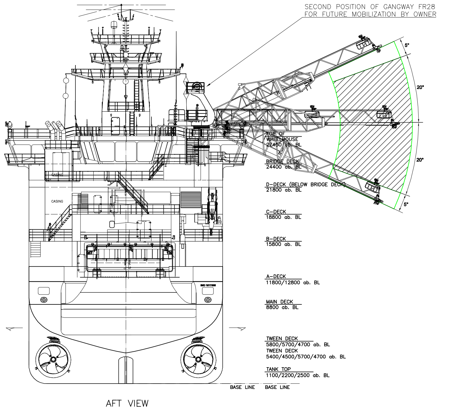
AFT VIEW
