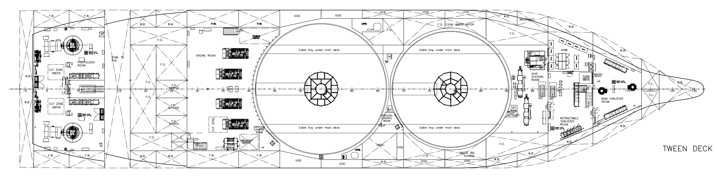
MAIN DECK
